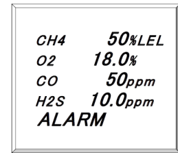
Second Alarm Setpoint Display (ALARM)
